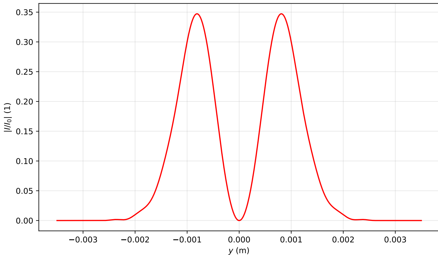
Intensity profile I(x=0, y, z=2.946)/I_0 , P_{in}=2.0P_{cr} , artificial time
